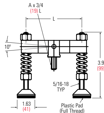
GH-YP-3160 Yoke attached to GH-12265 Clamp (Sold separately)
