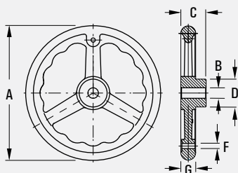
Handwheel Without Handle
